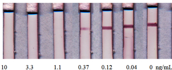
Fig. (7). The appearance of analytical zones of the strips after ICA of T2T when antibodies are in solution.
