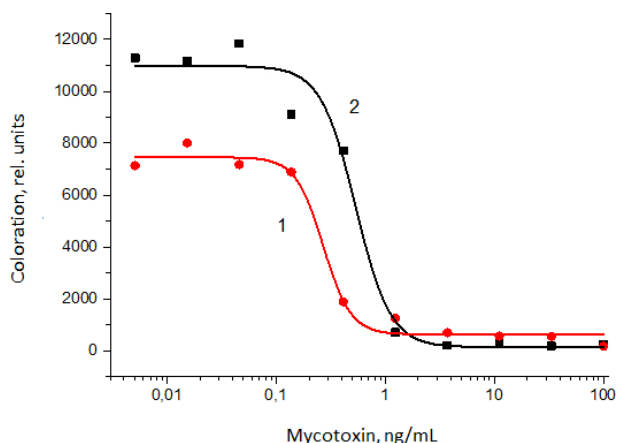
Fig. (5). Dependences of coloration intensity from the concentrations of AFB1 (curve 1) and T2T (curve 2) for stepwise ICA with indirect labeling. The presented colorations accord to mean values for n = 3; standard errors vary in the range from 8 to 15%.
