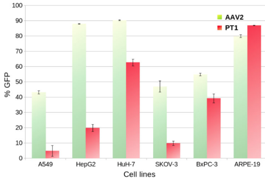
Fig. (2). In vitro transduction comparisons. Left: transduction efficiencies (percentage of GFP-positive cells) in the ARPE-19 cell line of PT1 compared with that of four control capsids. Right: comparison of transduction efficiencies of AAV2 and PT1 in six different cell lines. Error bars show standard deviation.
