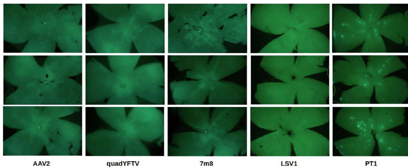
Fig. (5). Retinal flat mounts. Fluorescence microscopy images of three representative retinal flat mounts are shown for each variant (all images are available in the repository referenced in the Data availability section). From left to right: AAV2, quadYFTV, 7m8, LSV1, PT1. For LSV1 and PT1, exposure time was increased to make GFP expression more visible.
