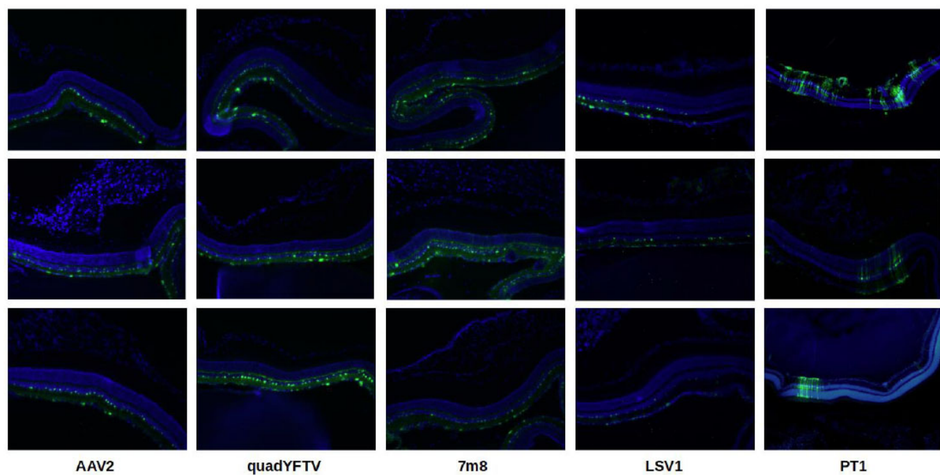
Fig. (6). Retinal cryosections. Fluorescence microscopy images of three representative retinal cryosections are shown for each variant (all images are available in the repository referenced in the Data availability section). From left to right: AAV2, quadYFTV, 7m8, LSV1, PT1.
