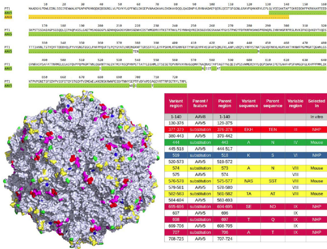
Fig. (1). Sequence features of capsid variant PT1. Top: amino acid sequence of PT1 capsid VP1 protein compared with parent capsids AAV8 (gold) and AAV5 (green). Dots indicate identity. Parental sequences are only shown when they differ from that of PT1. Bottom left: Three-dimensional model of AAV5 capsid showing the surface substitutions of PT1 color-coded according to their region (red: VR-III, green: VR-IV, blue: VR-VI, yellow: VR-VIII, magenta: VR-IX). Bottom right: detailed description of PT1 capsid VP1 sequence. Substitutions are color-coded in the same way as the model on the left.
