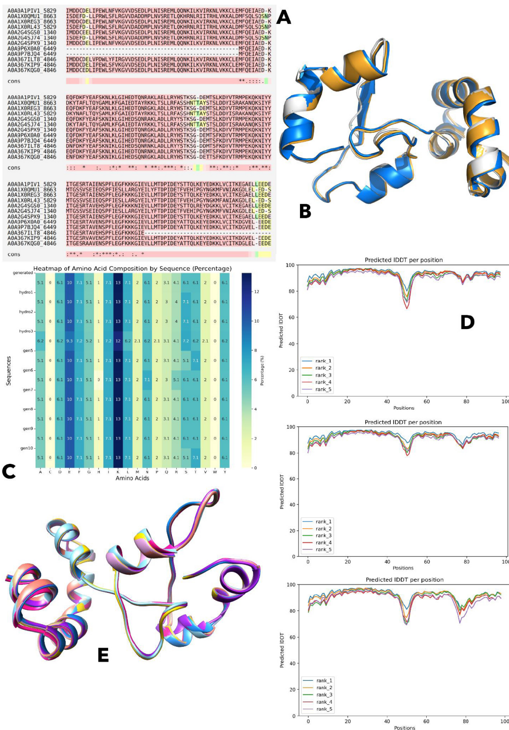
Fig. (1). (A) Multiple Sequence Alignment (MSA) highlighting the conserved region. (B) Structural visualization of the conserved regions identified in the MSA. (C) Amino acid composition of the ten generated de novo sequences. (D) Predicted high-quality structures selected based on pLDDT scores. (E) Superimposition of the generated protein structures to assess structural consistency.
