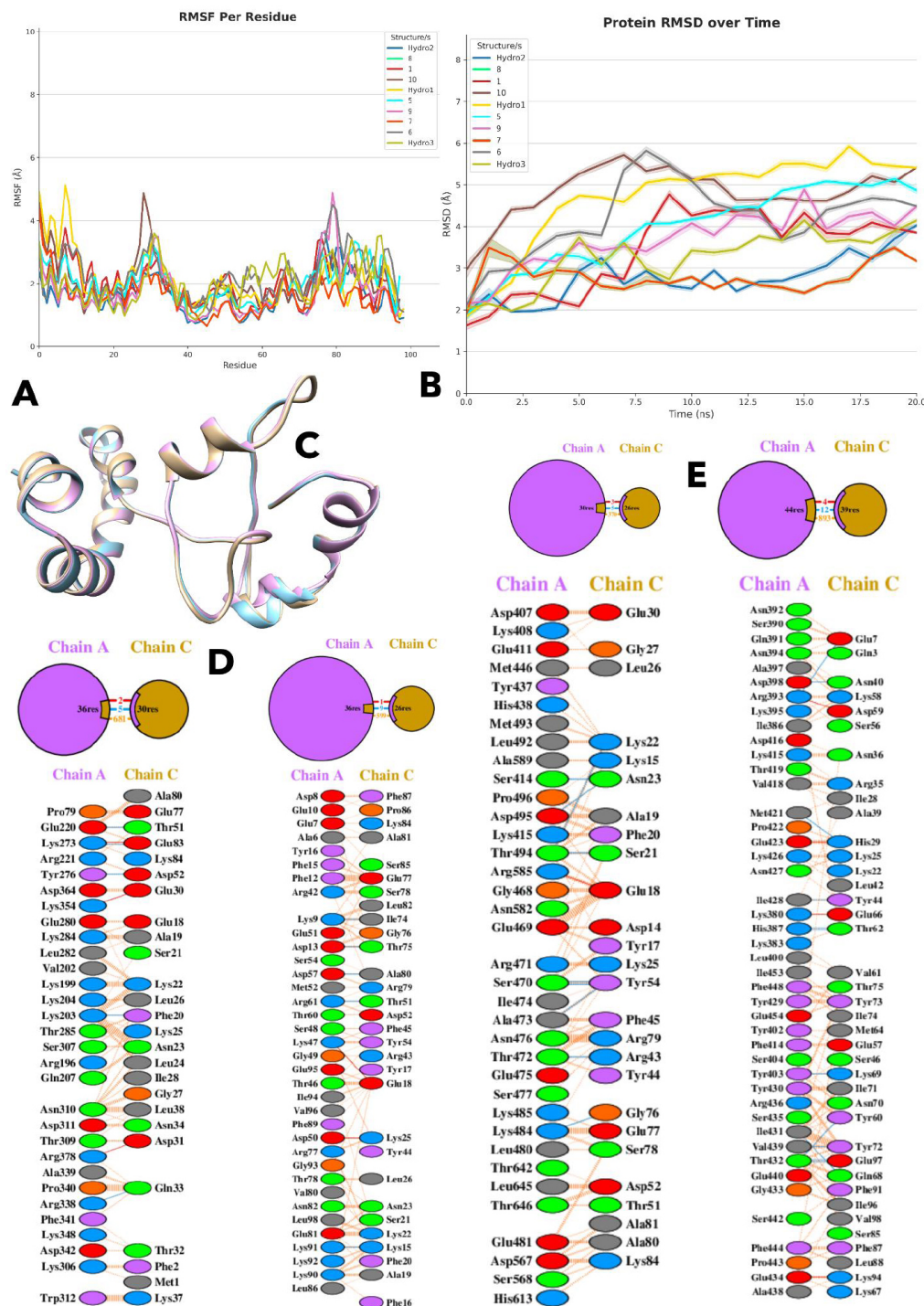
Fig. (2). (A) Root Mean Square Fluctuation (RMSF) analysis showing per-residue flexibility of the generated protein structures. (B) Root Mean Square Deviation (RMSD) plot indicating that structure 7 undergoes early conformational changes before stabilizing. (C) Superimposed structures of Hydro 2, Hydro 3, and structure 7, identified as the most stable during molecular dynamics simulations. (D) Hydrogen bonds and salt bridges formed between the de novo designed protein Gen7 and HSP90 from various fungal species and humans, indicating interaction specificity. (E) Number of interface residues involved in binding between Gen7 and HSP90 from different fungal species and human, reflecting interaction surface size.
